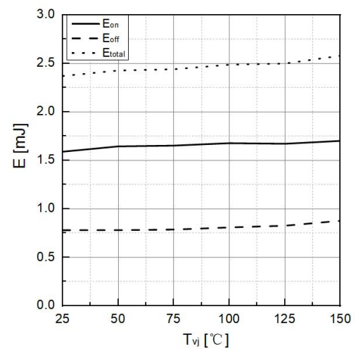
Fig 12. Typical switching energy losses as a function of T_{vj}
